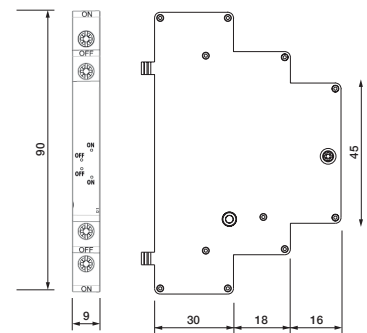
fig. 2. Dimensions (mm)
