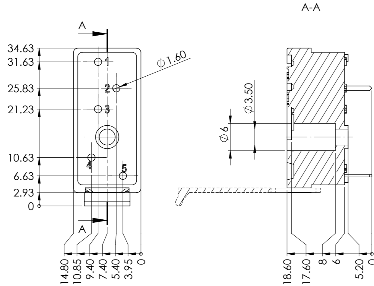
Bottom View
