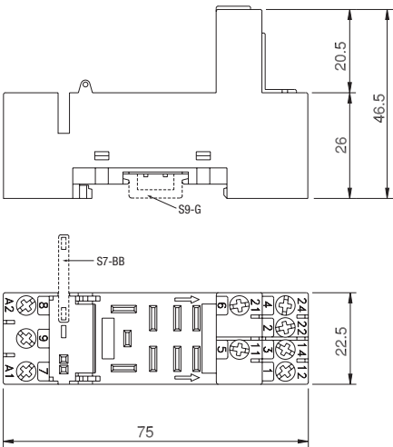
fig. 2. Dimensions (mm)
