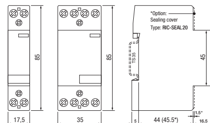
fig. 2. Dimensions (mm)
