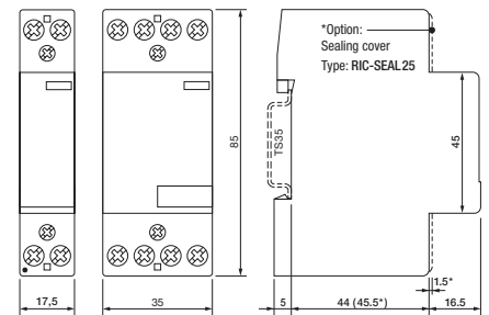
fig. 2. Dimensions (mm)
