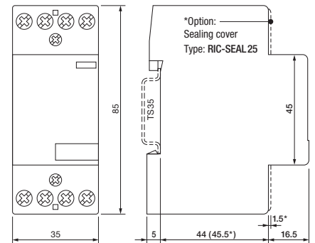
fig. 2. Dimensions (mm)
