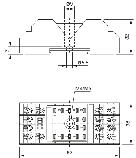
fig. 2. Dimensions (mm)
