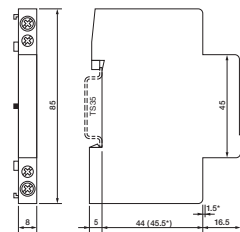
fig. 2. Dimensions (mm)
