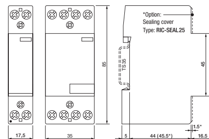
fig. 2. Dimensions (mm)
