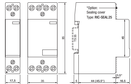
fig. 2. Dimensions (mm)
