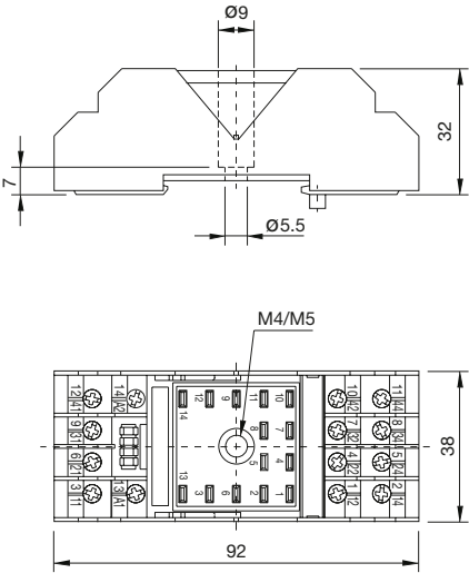
fig. 2. Dimensions (mm)
