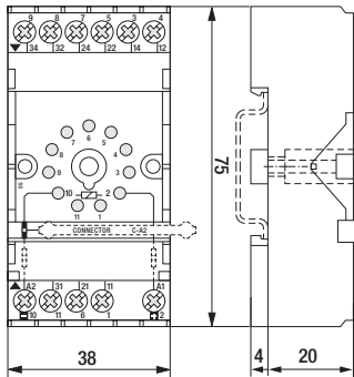
fig. 2. Dimensions (mm)
