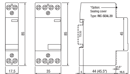
fig. 2. Dimensions (mm)
