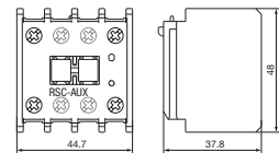
fig. 2. Dimensions (mm)
