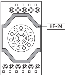
fig. 1. Mounting
