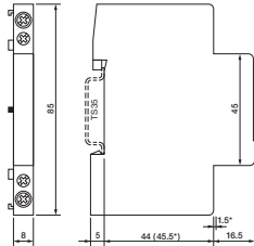
fig. 2. Dimensions (mm)
