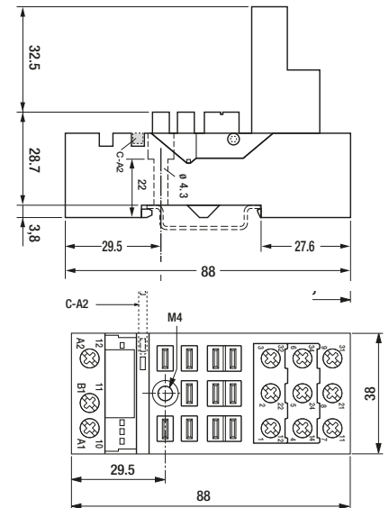
fig. 2. Dimensions (mm)
