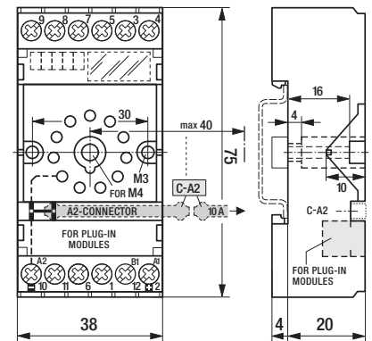
fig. 2. Dimensions (mm)
