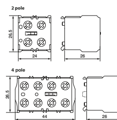
fig. 2. Dimensions (mm)
