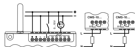
fig. 2. Max. breaking capacity RZ
